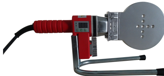
No. SHS 110.230V SHS110.110V
